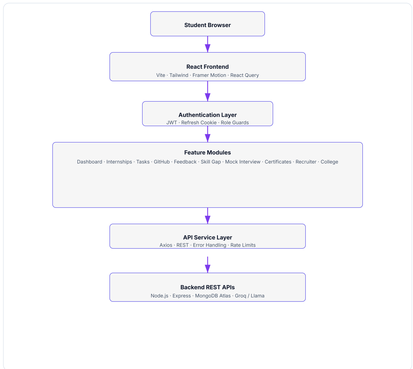
Figure 3 — Frontend application flow (student browser → frontend → auth → feature modules → API service → backend APIs)
