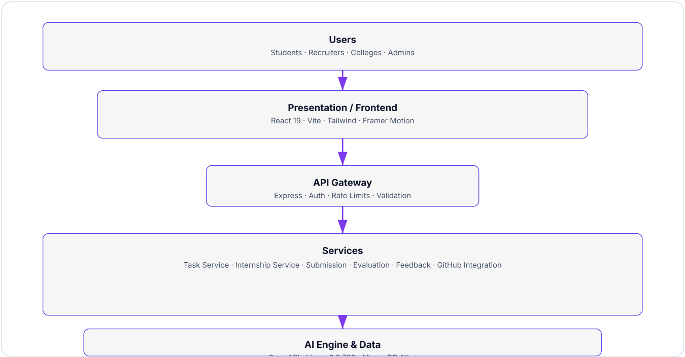
Figure 1 — InternX AI layered system architecture (Users → Presentation → API Gateway → Services → AI Engine & Data)
